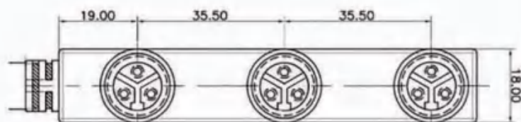
XYM15F-3P 1 to 3
