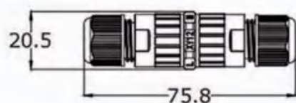
XY12-W01
