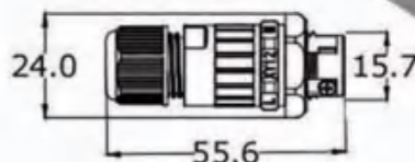
XY12-BPG9
