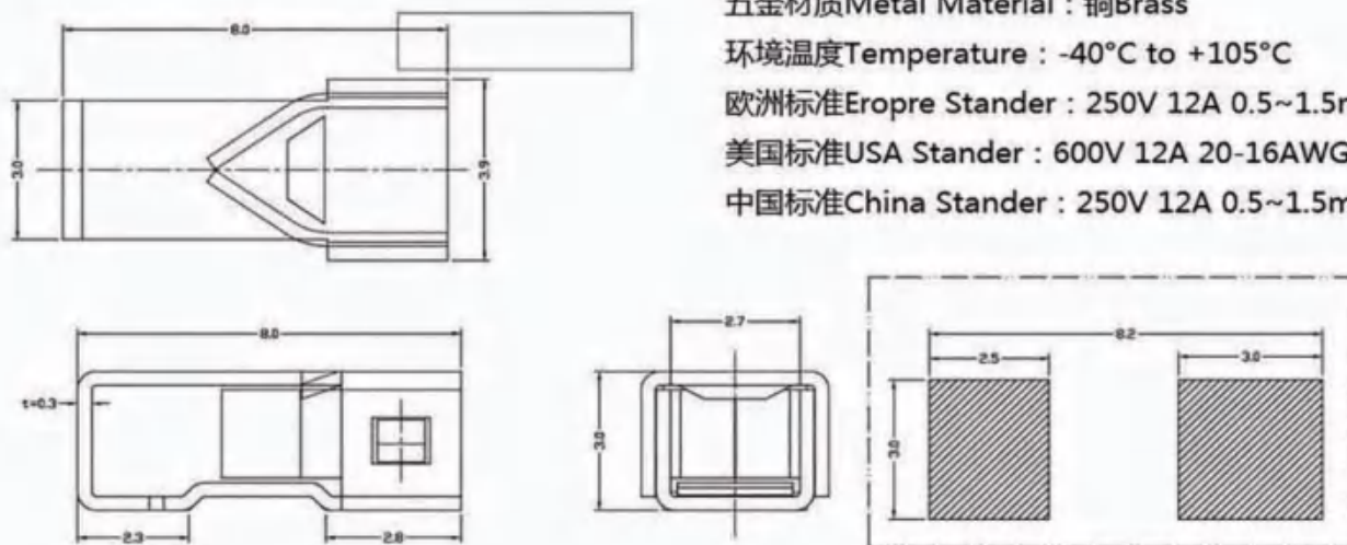
2065 LAYOUT
